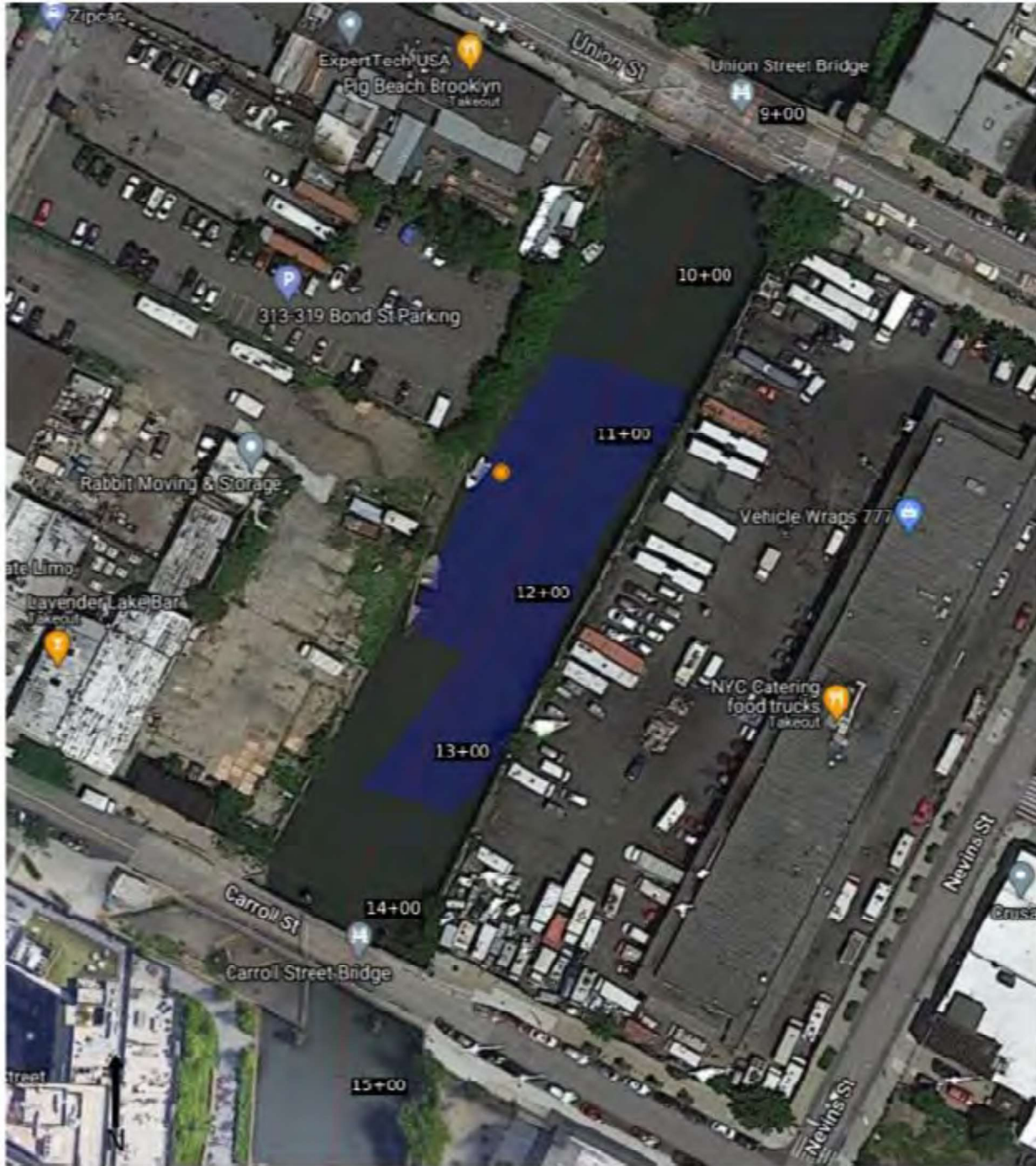
Figure 2 – Approximate Area Dredged between December 28, 2020 and December 31, 2020. Dredging was not conducted January 1, 2021. Figure Provided by the Trust.
